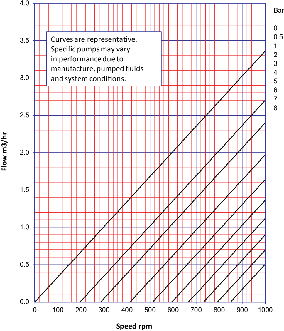
Flow at 1cPs
