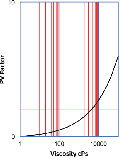
Power Viscosity Correction
