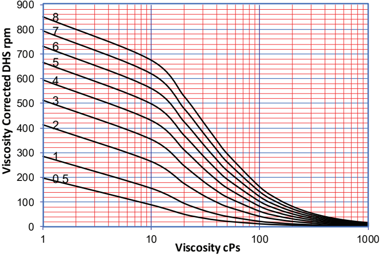
Flow - Viscosity Correction
