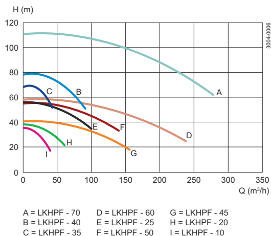
Figure 1. Frequency: 50 Hz, Speed (Synchr.): 3000 rpm
