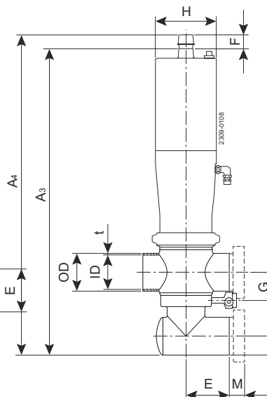
Figure 16. Shut-off valve with two valve bodies
