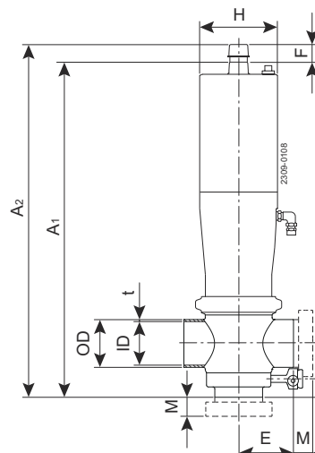
Figure 15. Shut-off valve with one valve body
