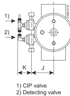
Figure 17. Top view
