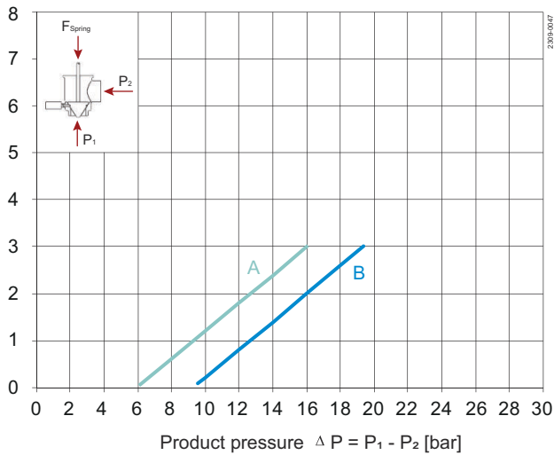
Figure 3. ø89 actuator
