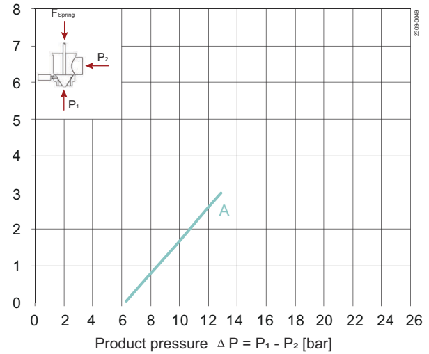
Figure 6. ø199 actuator
