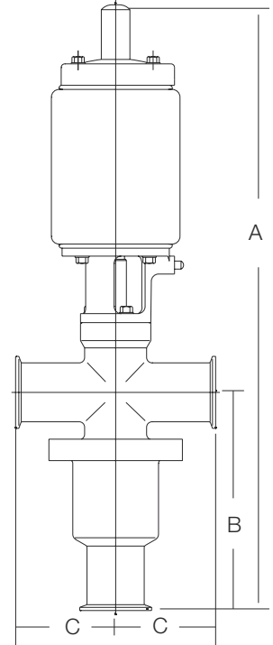
Figure 8. 761-47 Reverse-Acting
