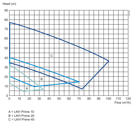
Figure 1. Frequency: 50Hz - Speed (synchr): 3000 rpm
