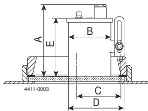
Sight glass LKS 105 with miniVISION type 53.
