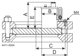
Sight Glass acc. to DIN 28120 with miniVISION type 53.
