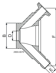
Figure 4. Valve body: Tank welding
