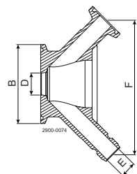
Figure 3. Valve body: Tri-clamp
