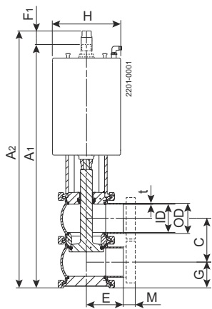
Figure 1. Shut-off valve
