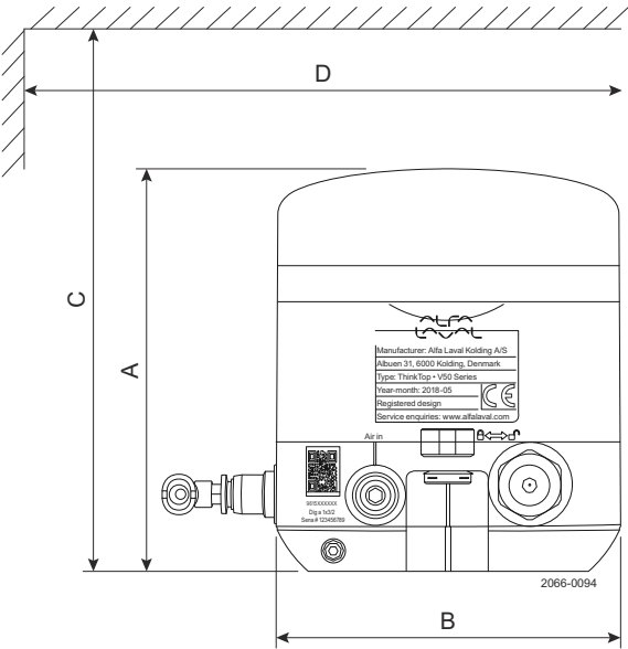
Figure 1. ThinkTop V 50
