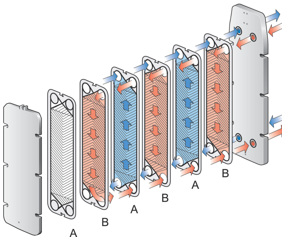
Example of a single-pass set up with gaskets facing the pressure plate.
