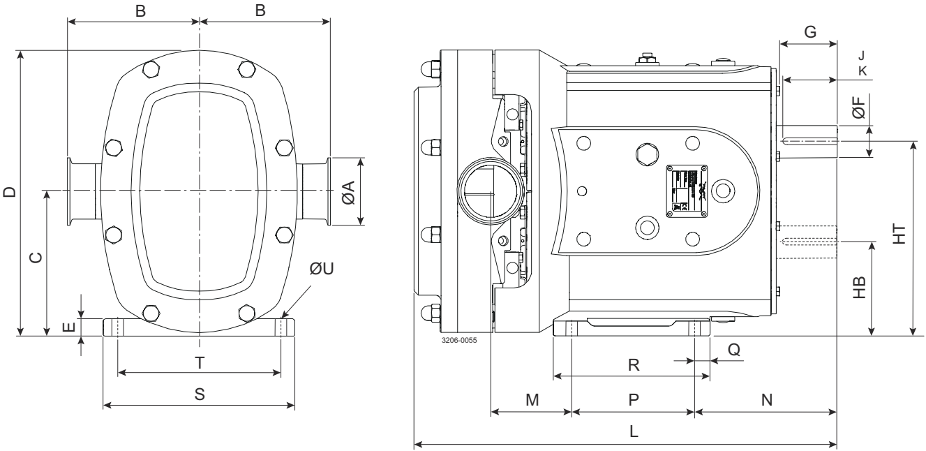
Figure 1. Horizontally ported
