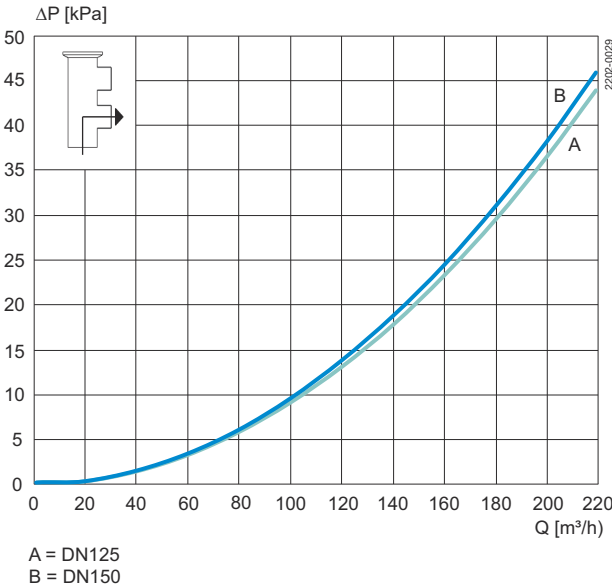
Figure 6. Change-over valve
