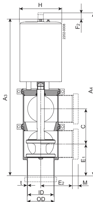
Figure 2. Change-over valve
