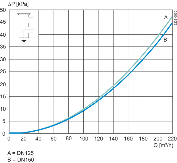
Figure 5. Change-over valve
