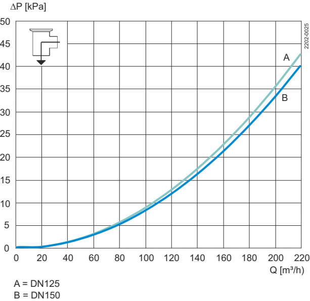
Figure 3. Shut-off
