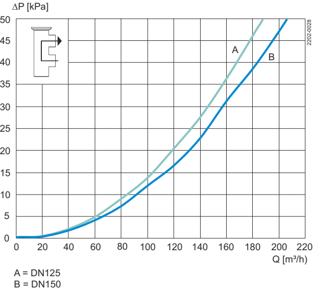
Figure 7. Change-over valve
