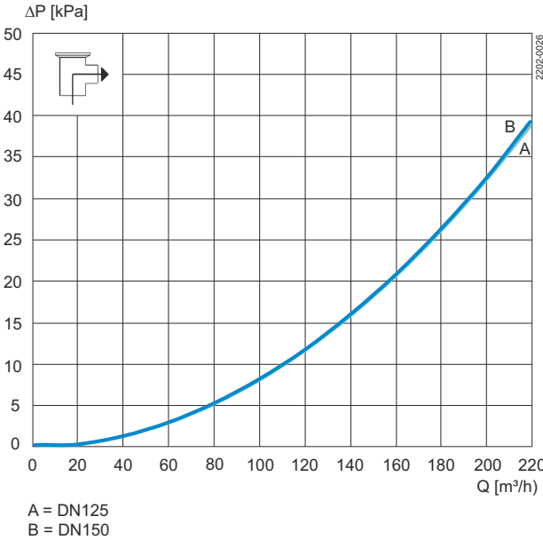
Figure 4. Shut-off
