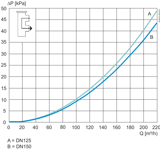
Figure 8. Change-over valve
