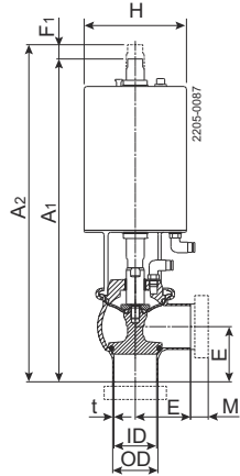
Figure 1. Shut-off valve
