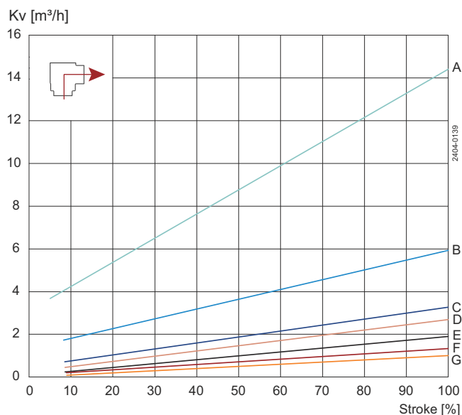
Figure 1. Valve size ISO 1"
