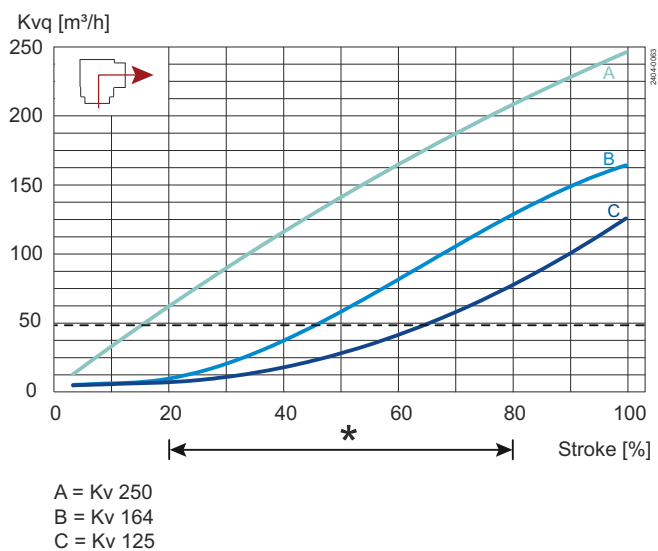
Figure 7. Valve size ISO 4"/DN100
