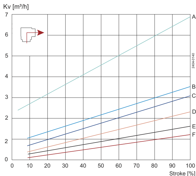
Figure 2. Valve size DN25
