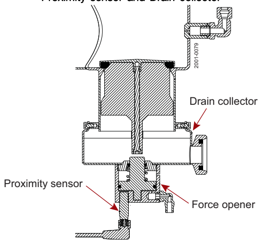
Cross section of Anti Vacuum House with Force opener, Proximity sensor and Drain collector
