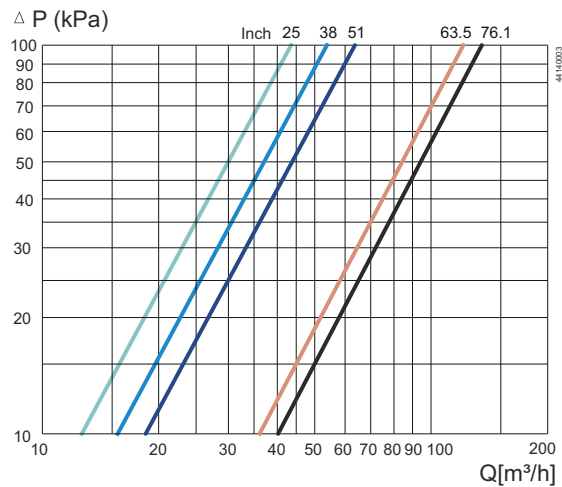
Figure 1. LKVF with \phi 0.079 in holes in filter element. Medium: water (68 °F).
