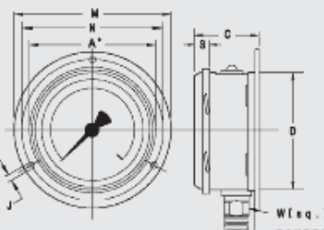
Rear flange
