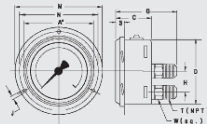
Front flange
