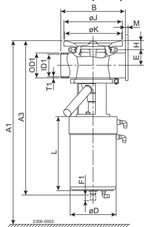
Figure 4. Unique-TO connected to tank flange
